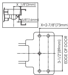
A : For wide stile door
