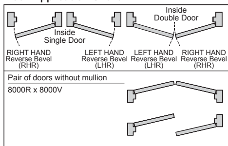
Door Application Chart
