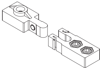
ZAB-D026-62 • Hold-open device • For track arm & rail: ZAR-I040
